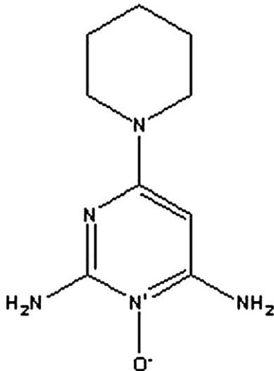
Fig 1. Minoxidil molecule.
