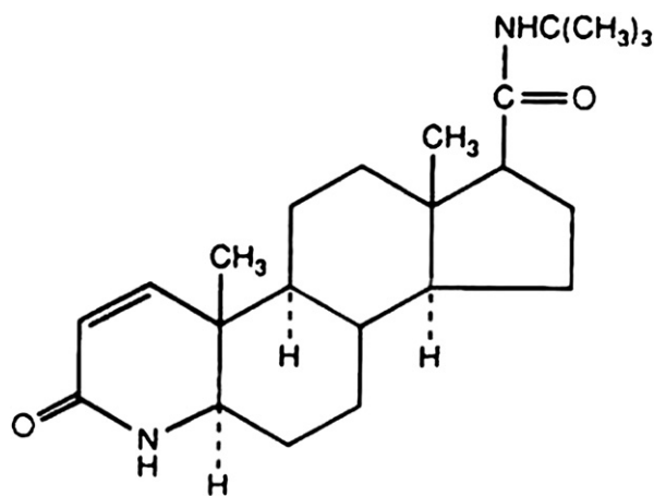
Fig 3. Finasteride molecule.
