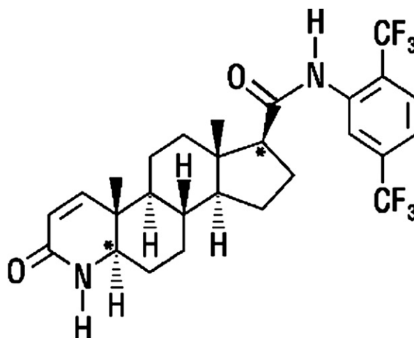
Fig 7. Dutasteride molecule.
